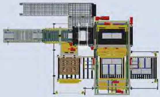
Type 1800 – up to 2000 bags/hr Configuration identical with Model 1500, additionally with a second row pusher (Guide A). Position over the gripper.
